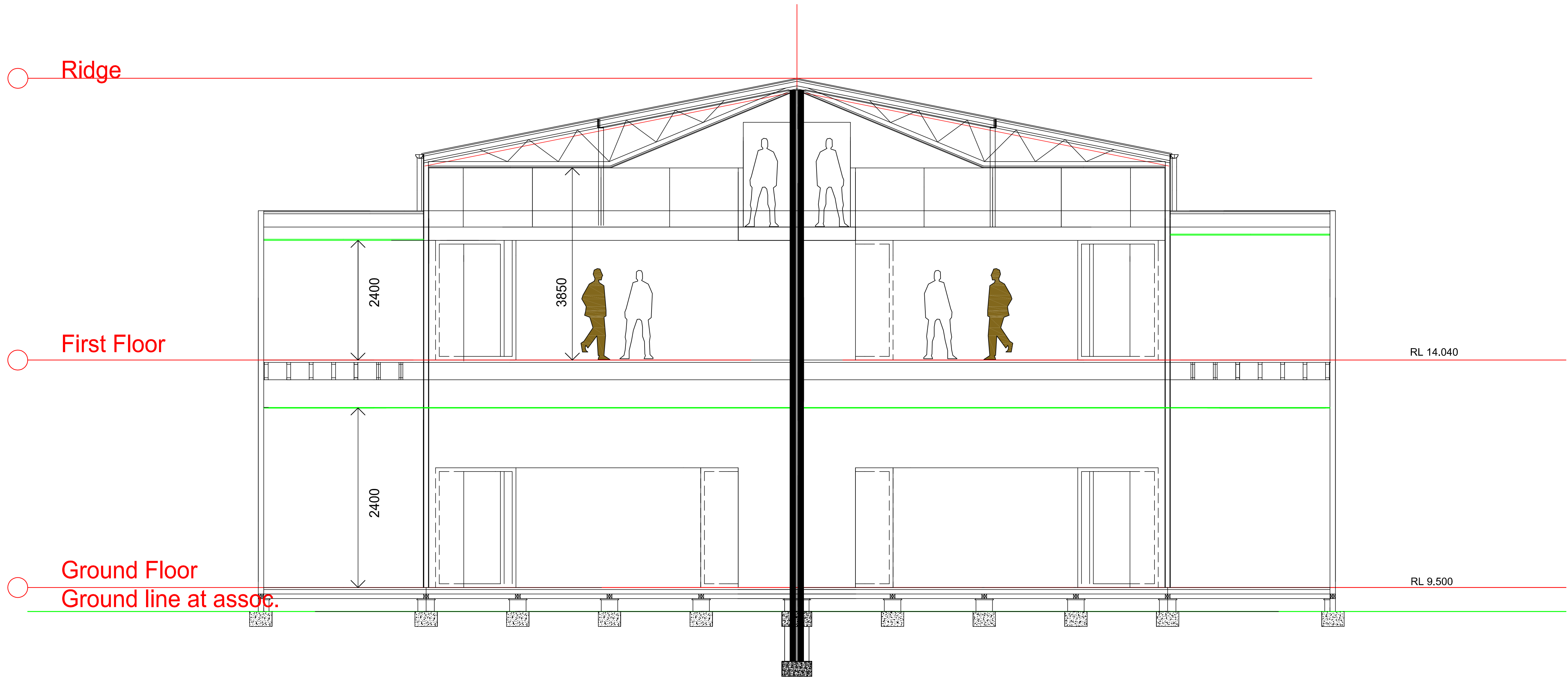
SECTION D - D
